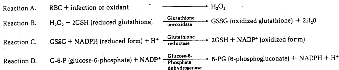
Figure 2-17. Reactions within erythrocytes to prevent accumulation of oxidants.
