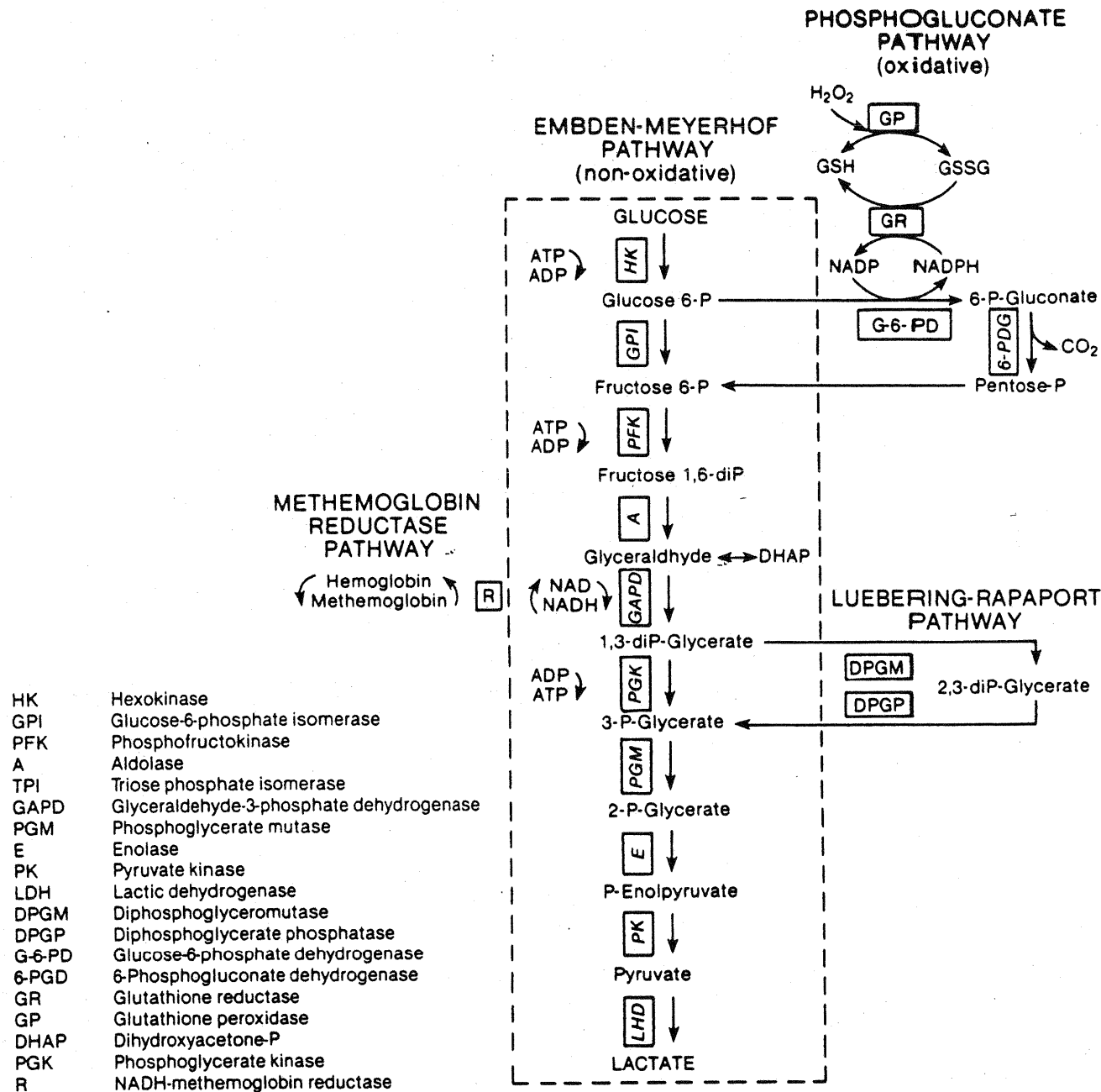
Figure 2-16. Red cell metabolism. (From Hillman, RS and Finch, CA: Red Cell Manual, ed 4. FA Davis, Philadelphia, 1974, with permission.)
